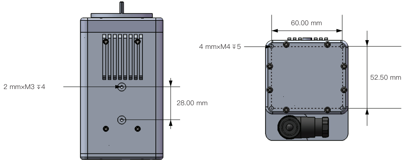
Figure 3. Detector Mechanical Drawing
