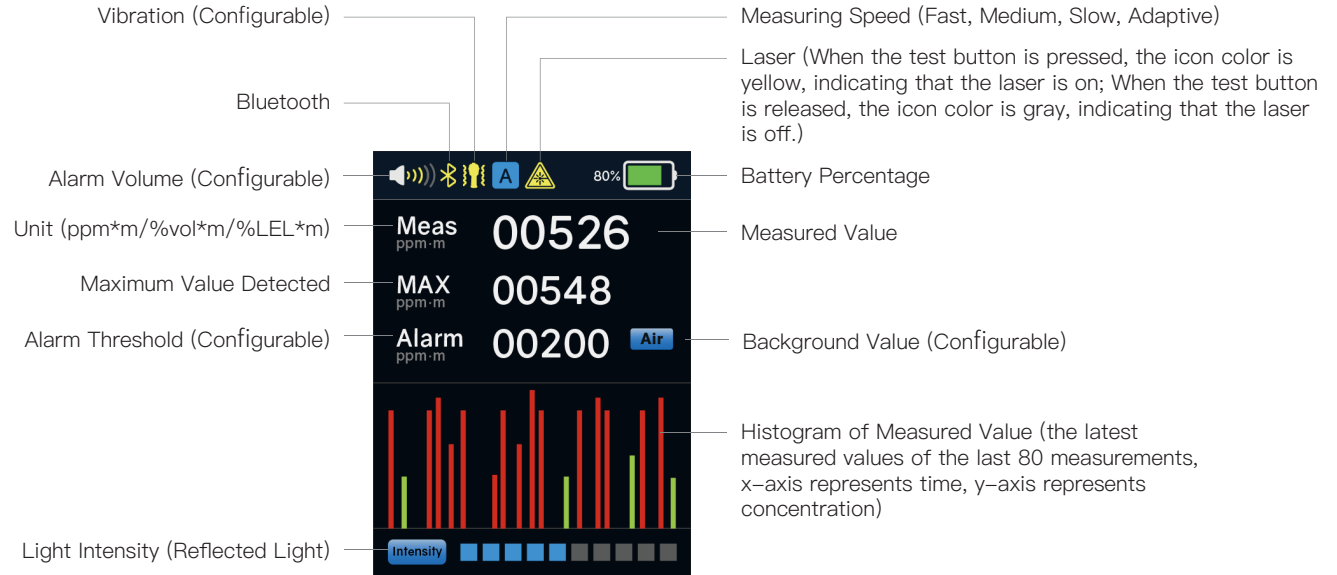
Figure 3.3 User Interface
