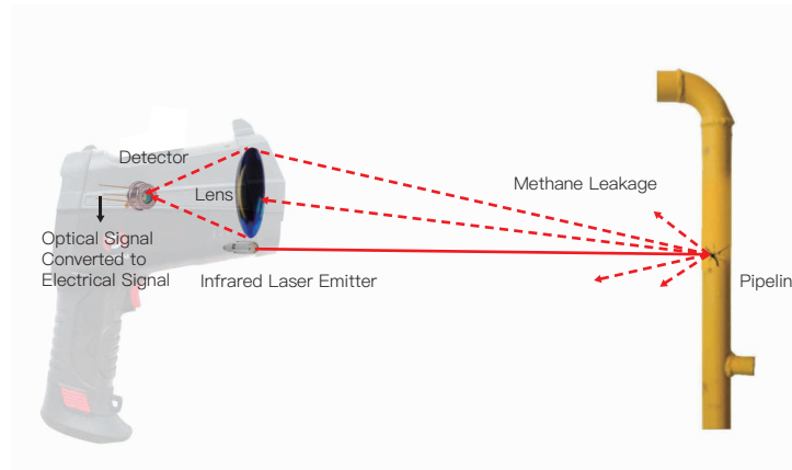
Figure 2.1 Working Principle
