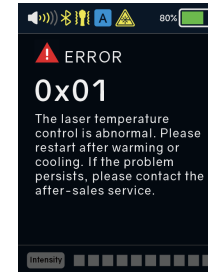
Figure 5.1 Error Messages
